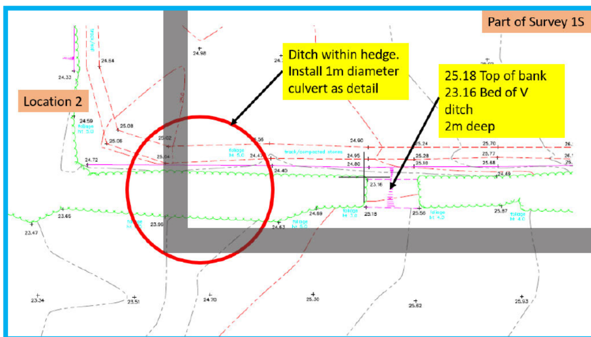
Location 2 Crossing of ditch and installation of culvert – Land Drainage Consent required.
