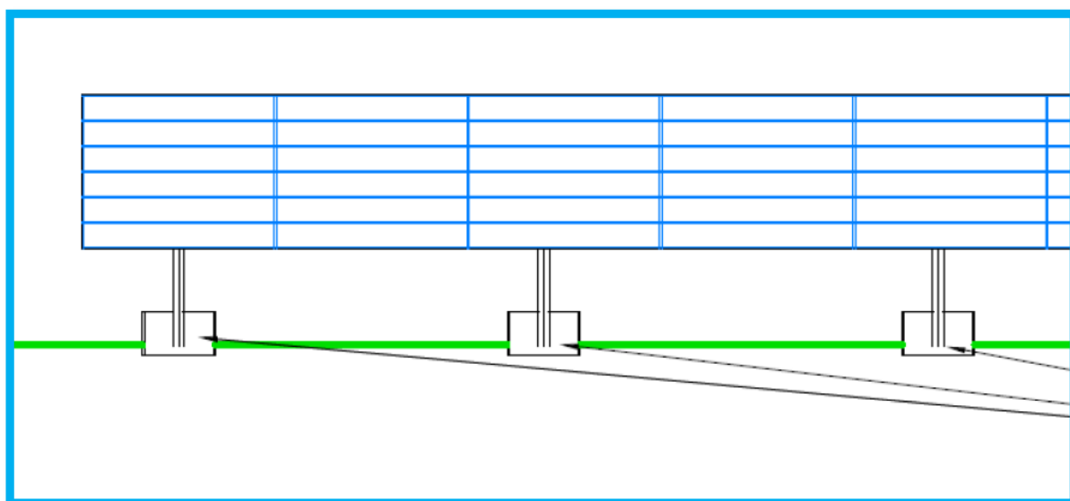
Fig 14 Elevation of array in green archaeological area showing minimal impact of pads on permeable soil.
