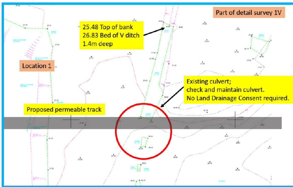
Location 1 No change to culvert – maintain existing - no Land Drainage Consent required.
