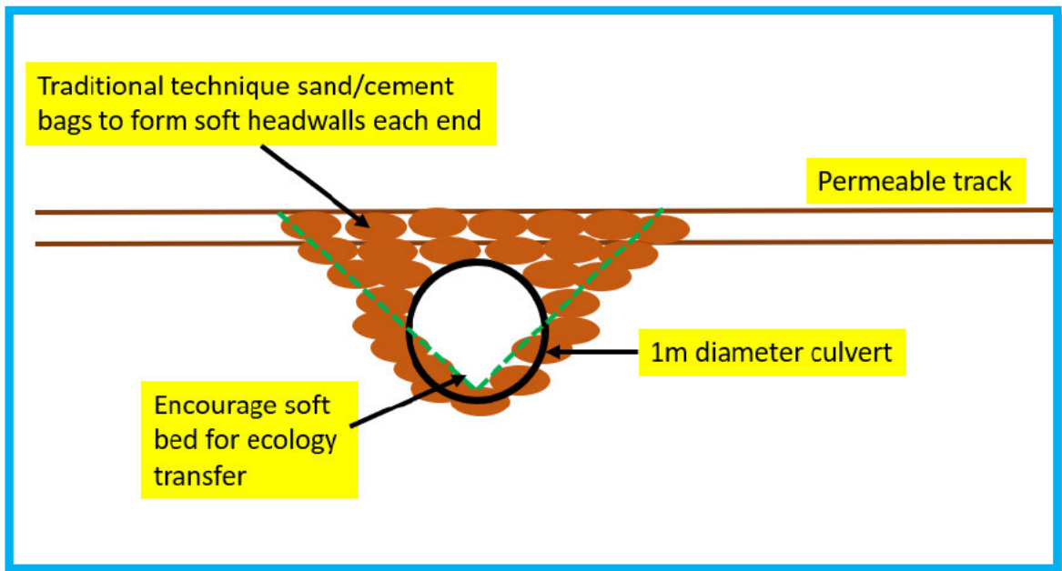
Location 2 Proposed detail of Culverted ditch.
