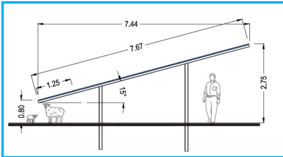
Fig 9 Typical section through array. Height dimensions will vary with undulations in the ground.
