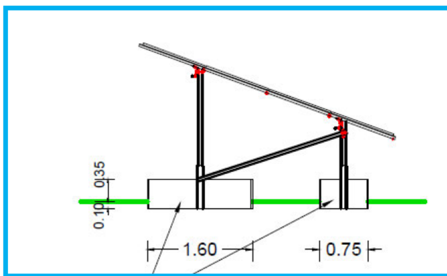
Fig 13 Cross section through array in the archaeological no-dig zone showing concrete pads.
