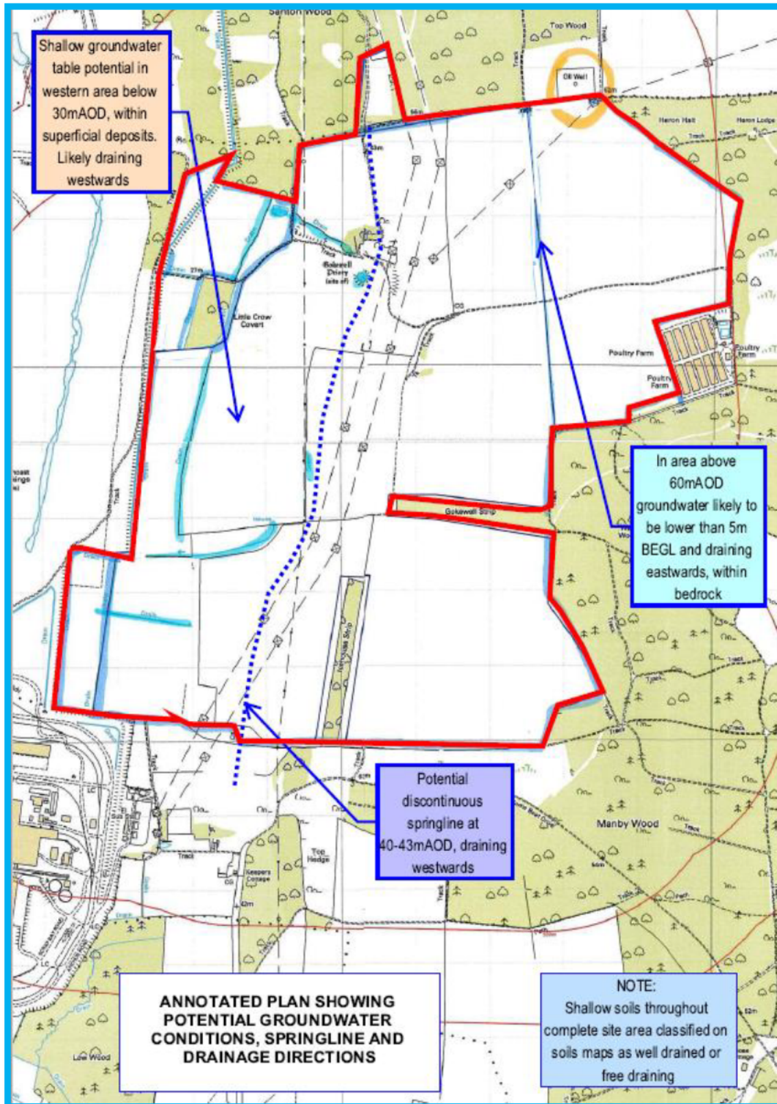
Fig 17 Extract from Integrale’s Phase 1 Ground Conditions Desk Study (Document 7.4 LC TA 3.2) showing the spring line and proposed Battery Energy Storage System Works No. 2A to the east (uphill) of the spring line. (The red outline is indicative of the study area used for Integrale’s report and does not represent the Order Limits).
