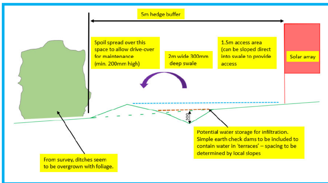
Fig 20 Typical swale formed with ridge and furrow technique and vegetated on completion. Ridge to be located on downhill side.
