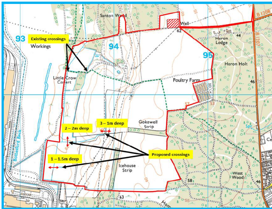
Fig 11 Track crossings labelled 1 (no longer required), 2 and 3, with the depths of the ditches crossed. See Appendix 1 for details.
