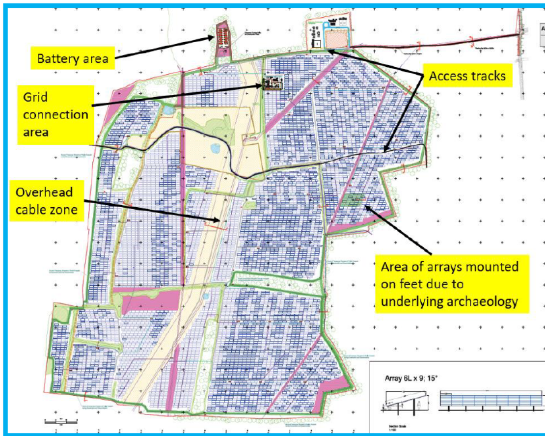
Fig 12a Extract from Works Details – Whole Site Plan (Document Ref 2.10 LC DRW). Note location of Battery Energy Storage System Works No. 2A to the north of the Order Limits.
